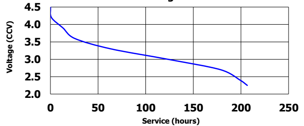
3.9 ohm Continuous Discharge
